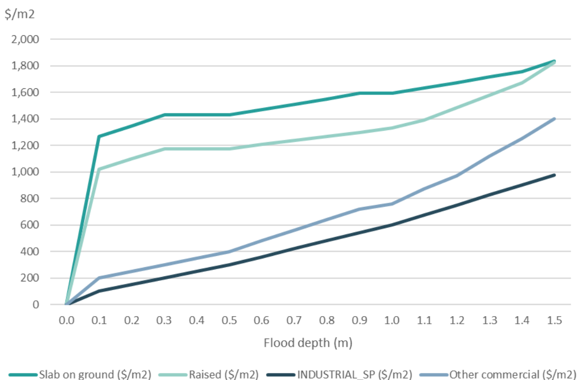
Figure 45. Estimated direct stage-damage curves for buildings ($/m 2 )
