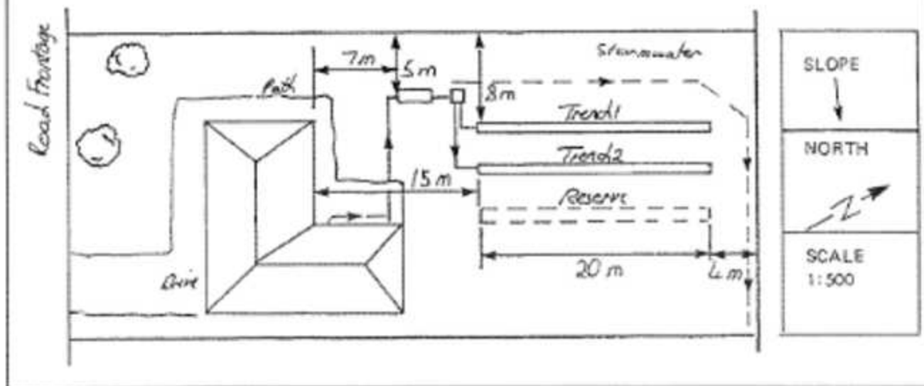
FIGURE 6.1 EXAMPLE RECORD SHEET – SEPTIC TANK AND TRENCH SYSTEM
