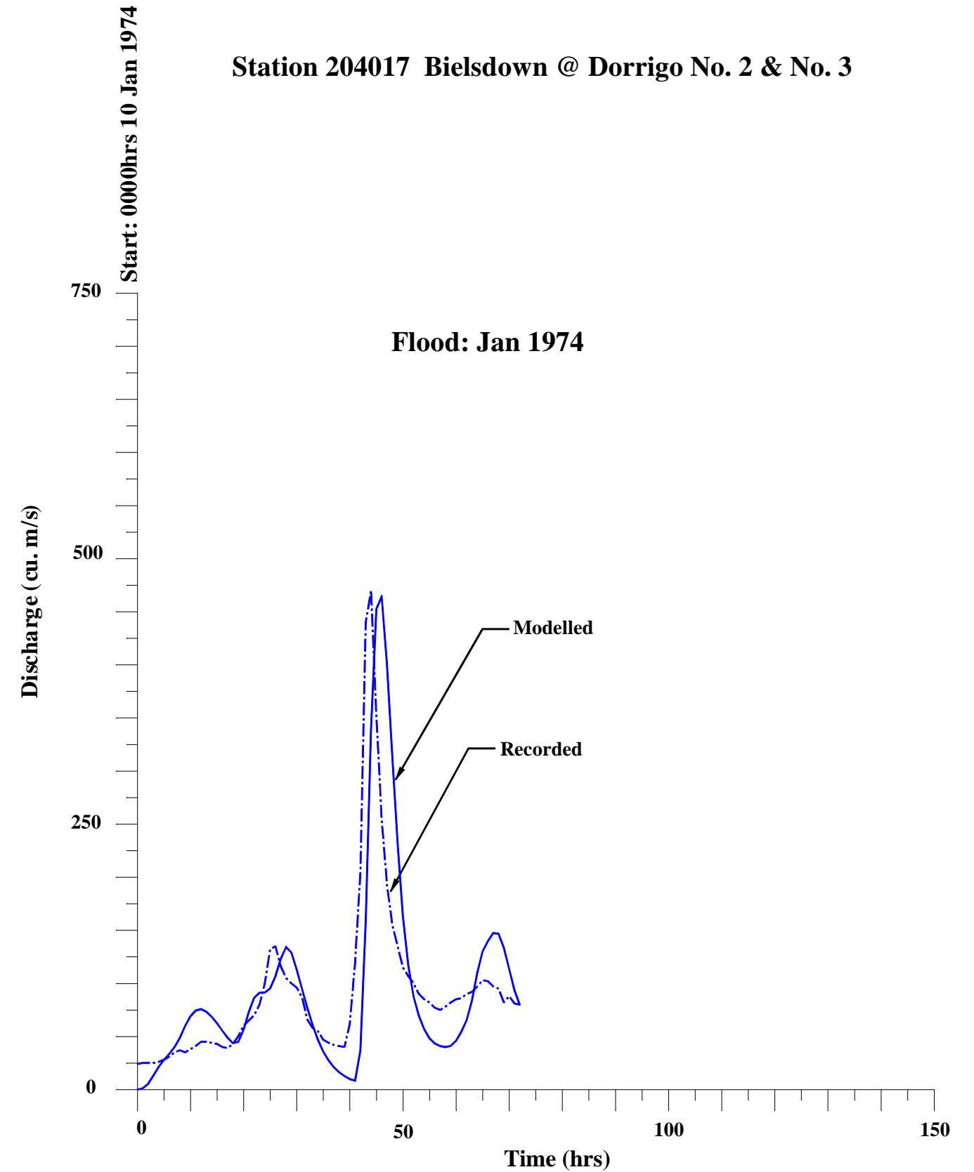
FIGURE 7 COMPARISON - 1973 & 1974 FLOODS
